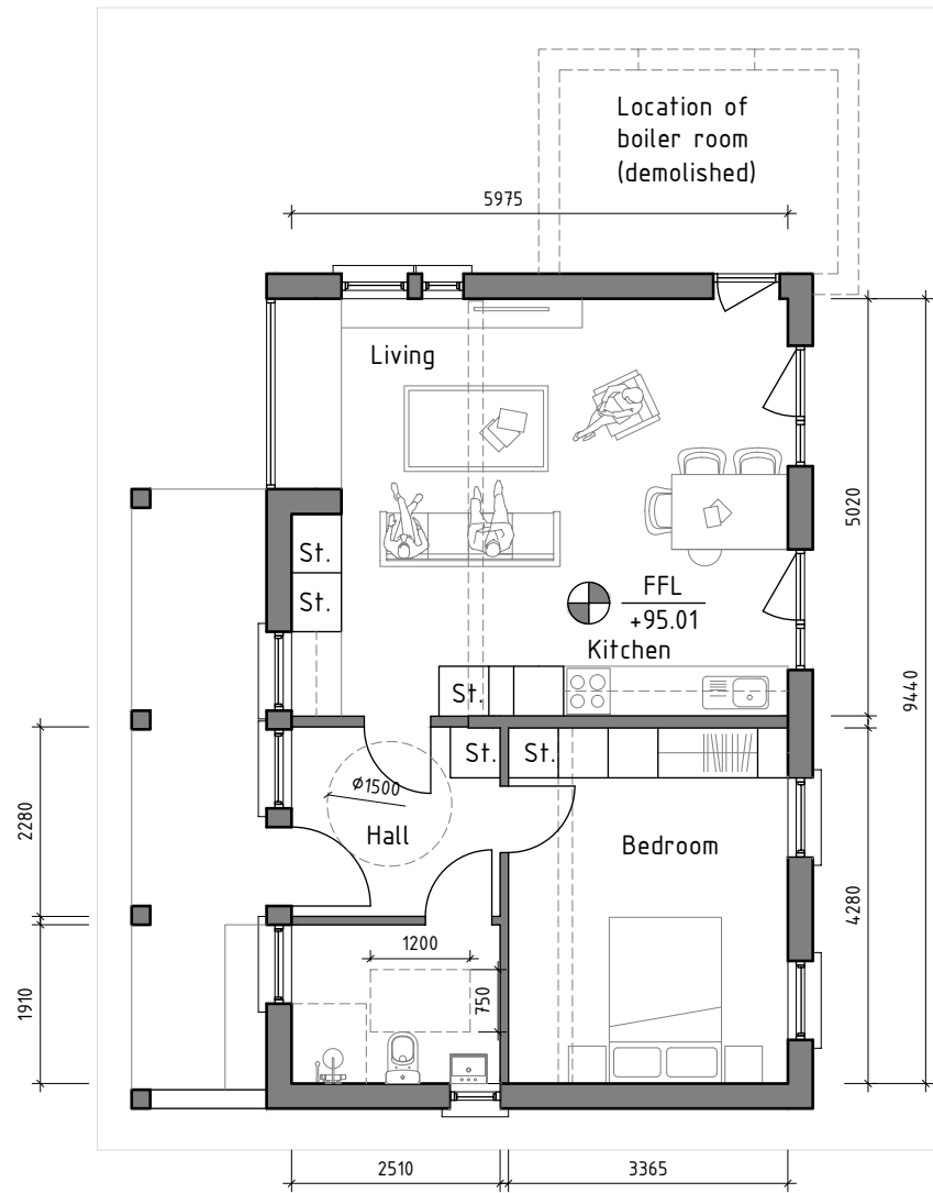
1 1-BED FLOOR PLAN PROPOSED 1:100@A3
